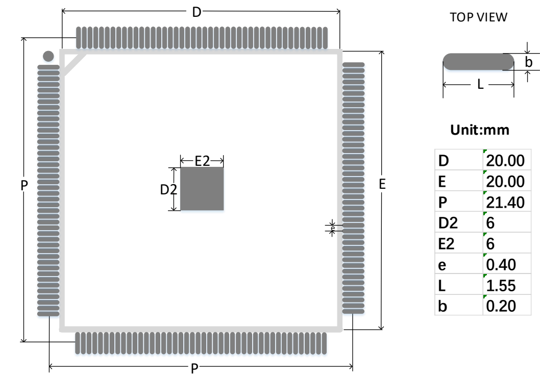
Figure 4-6 Recommended PCB Layout EQ176
