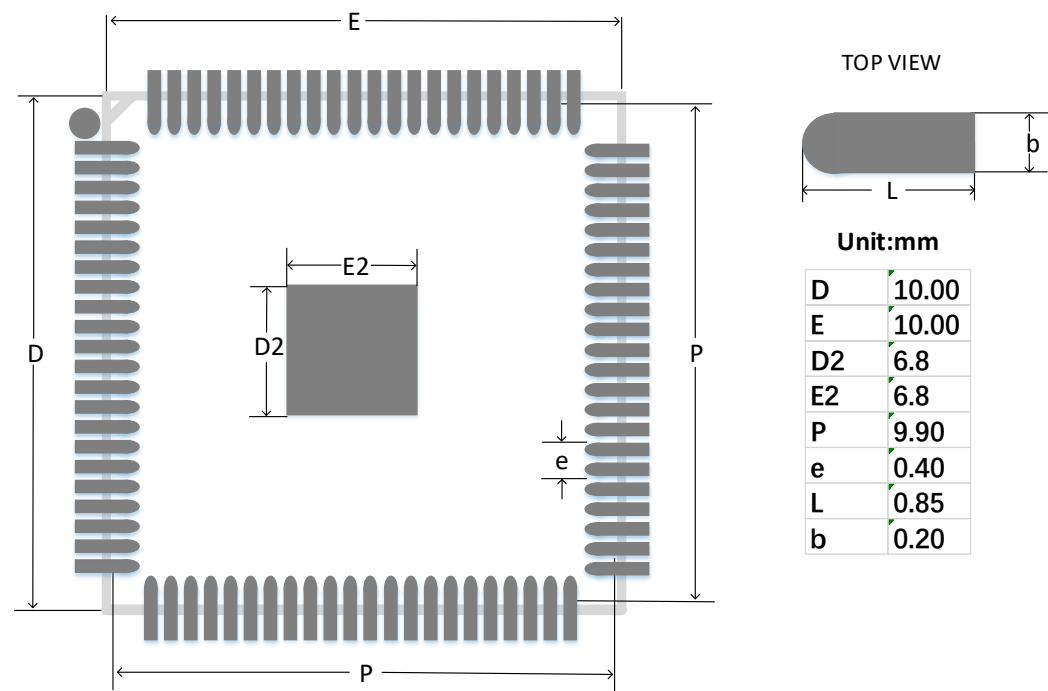
Figure 4-2 Recommended PCB Layout QN88/QN88P/QN88PF
