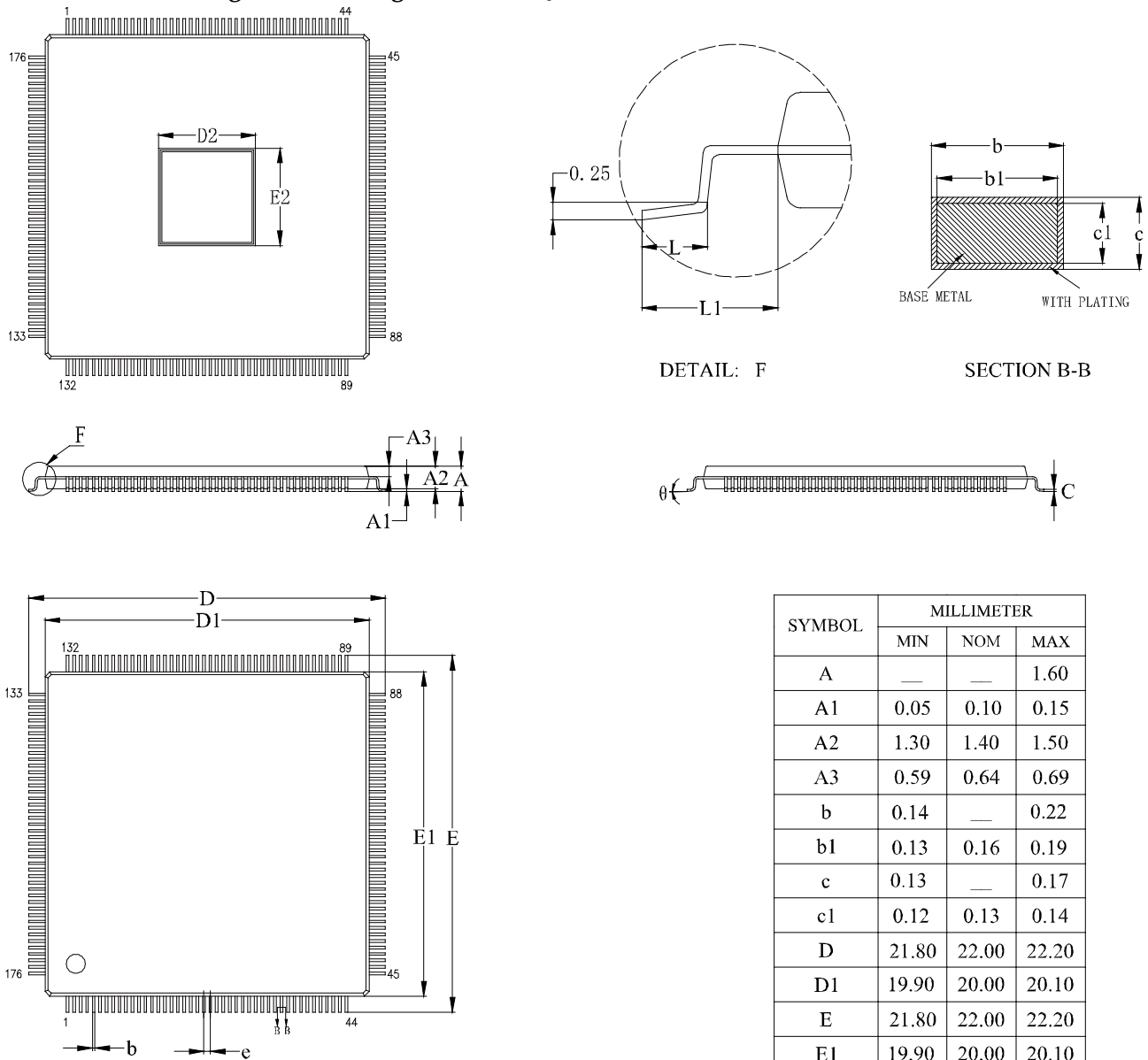
Figure 4-5 Package Outline EQ176
